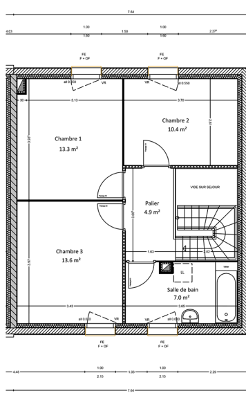
PLAN R+1
